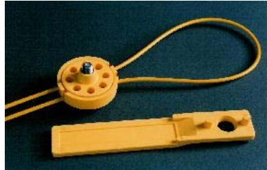
Optional use of padlocks (maximum 6mm shackle diameter) or seals for evidence of tamper.
